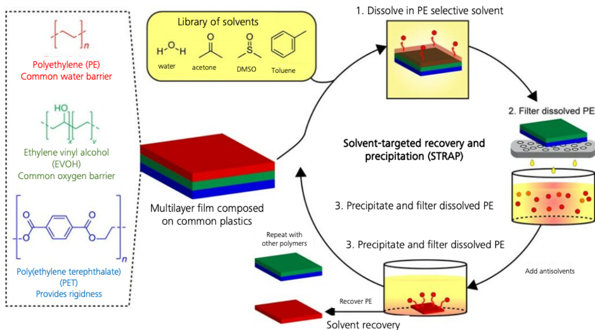
Figure 4: Three basic stages of the Solvent-Targeted Recovery and Precipitation (STRAP) process (Walker et al. 2020).
