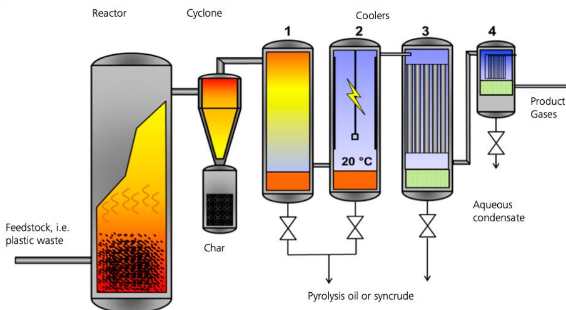
Figure 3: A general layout of the pyrolysis process including reactor, cyclone, and condensation stages (Pandey et al. 2019: 2533)
