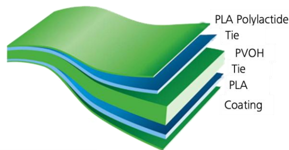
Figure 1: Multilayer film for Cheese or fresh pasta packaging with six layers (Food and Drink Business News 2021)
