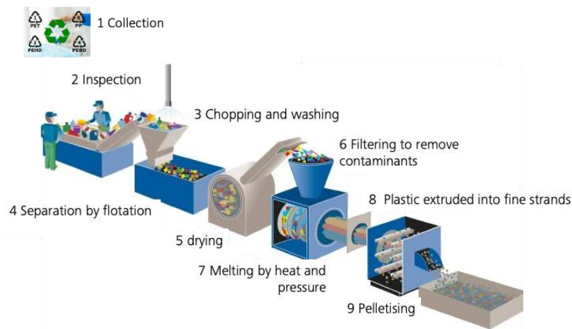
Figure 2: The steps of mechanical plastic recycling (Alberta Plastics Recycling Association 2025)
